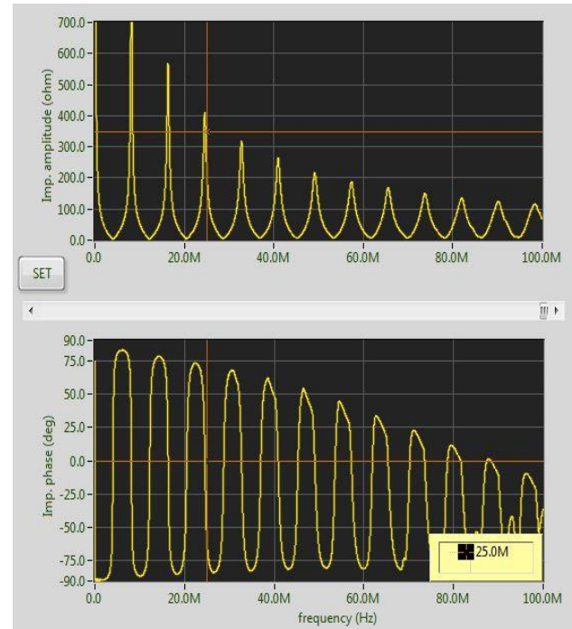
Fig. 1 Impedance of an unmatched transmission line
