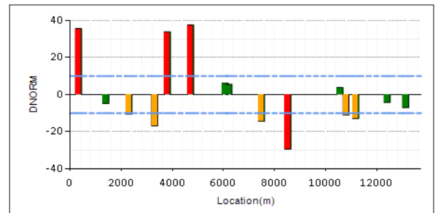
Fig. 12 Final DNORM graph quantifying each joint's condition
