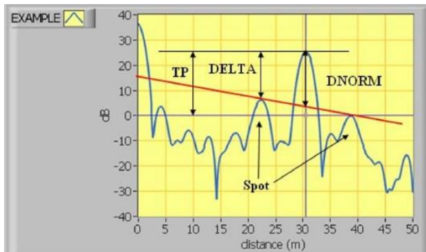
Fig. 3 HotSpot assessment with LIRA
