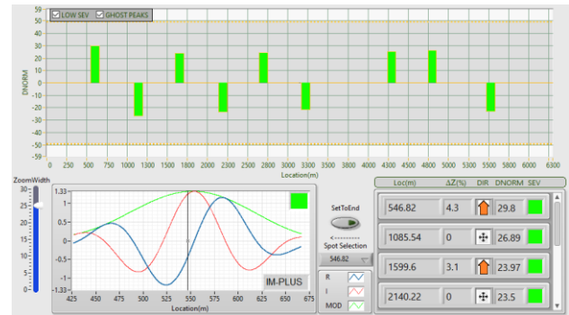
Fig. 4 DNORM graph of a 6.3 km. cable
