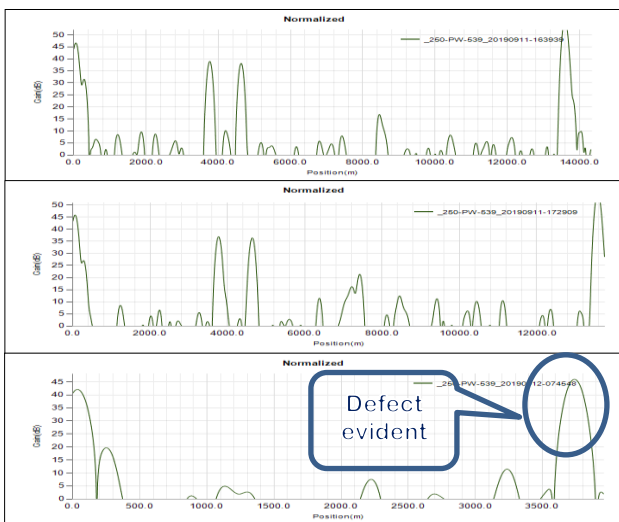
Fig. 11 Initial LIRA Spot Signature
