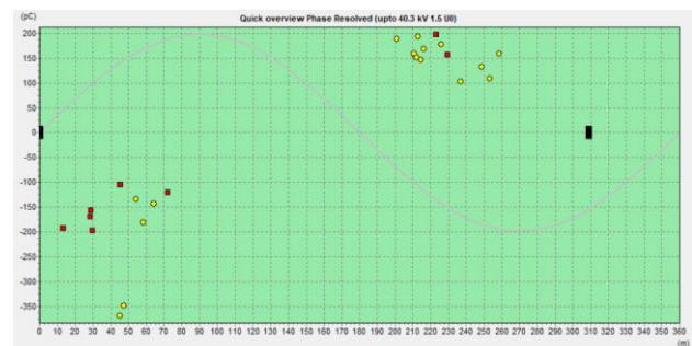
Fig. 8 Damped AC PRPD at 1.5U 0
