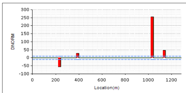
Fig. 14 Final DNORM graph - after burn-on-arc
