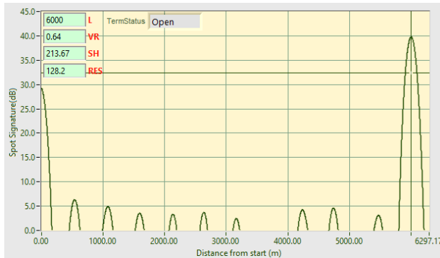
Fig. 2 Spot Signature graph of a 6.3 km. cable
