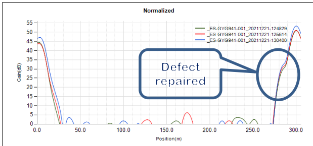
Fig. 10 Final LIRA Spot Signature
