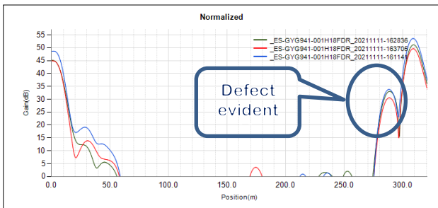
Fig. 9 Initial LIRA Spot Signature
