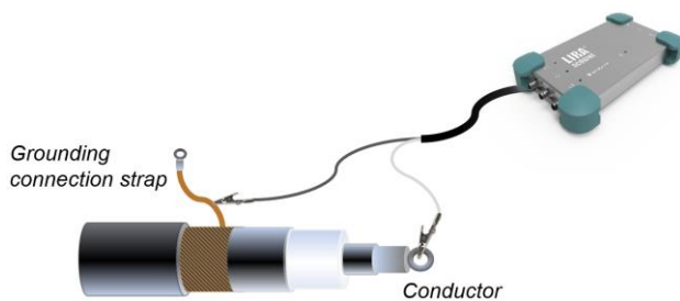
Fig. 7 LIRA connection set-up
